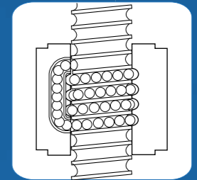
Z-AXIS BALL SCREW Precision movement
